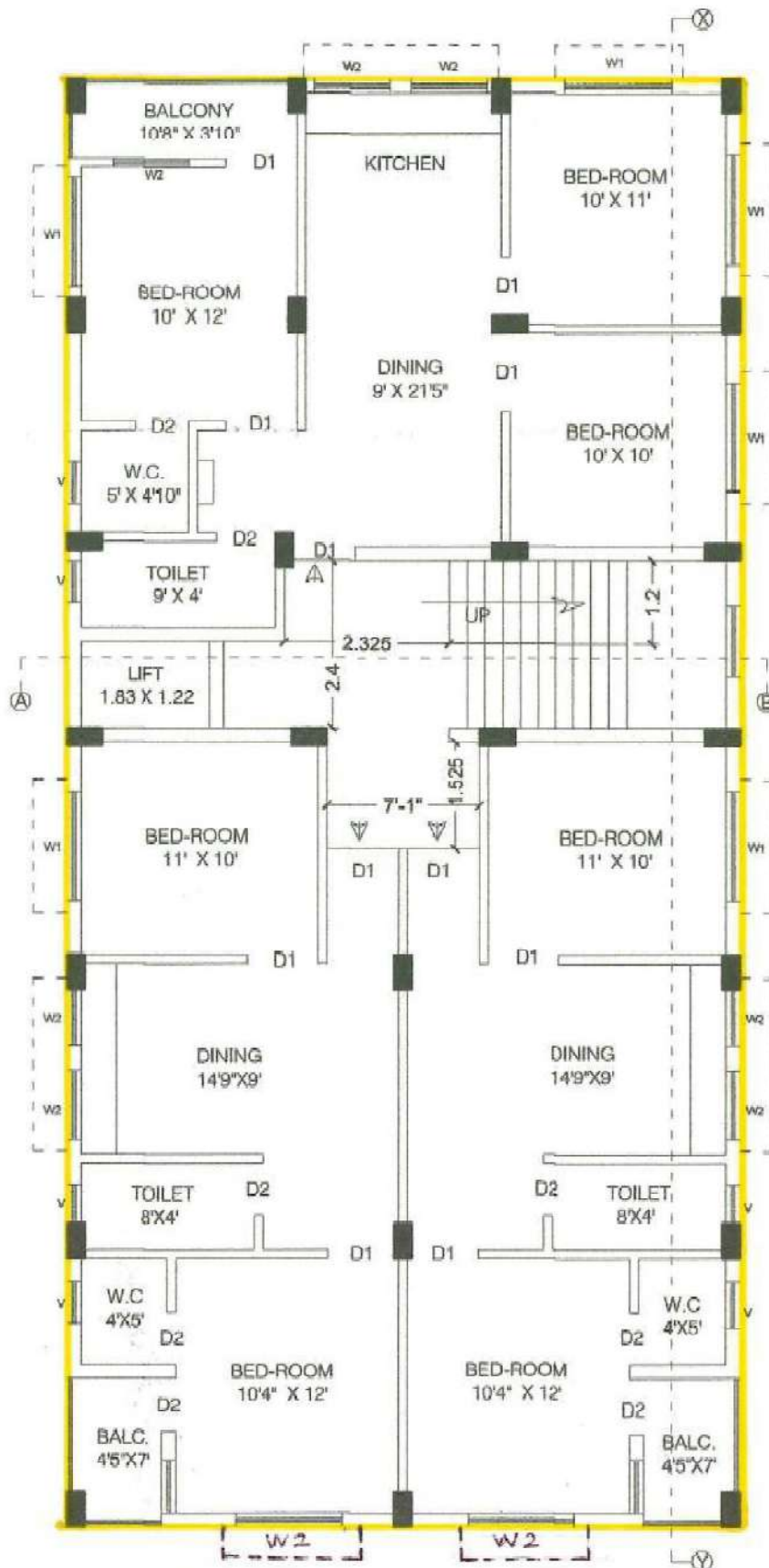
EXISTING TYPICAL FLOOR PLAN [ 1ST-4TH FLOOR ]
